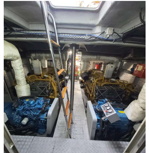
ENGINE ROOM
